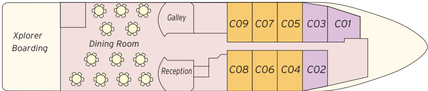
MAIN DECK
